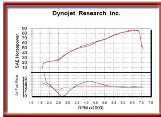
AIR FUEL RATIO GRAPH
